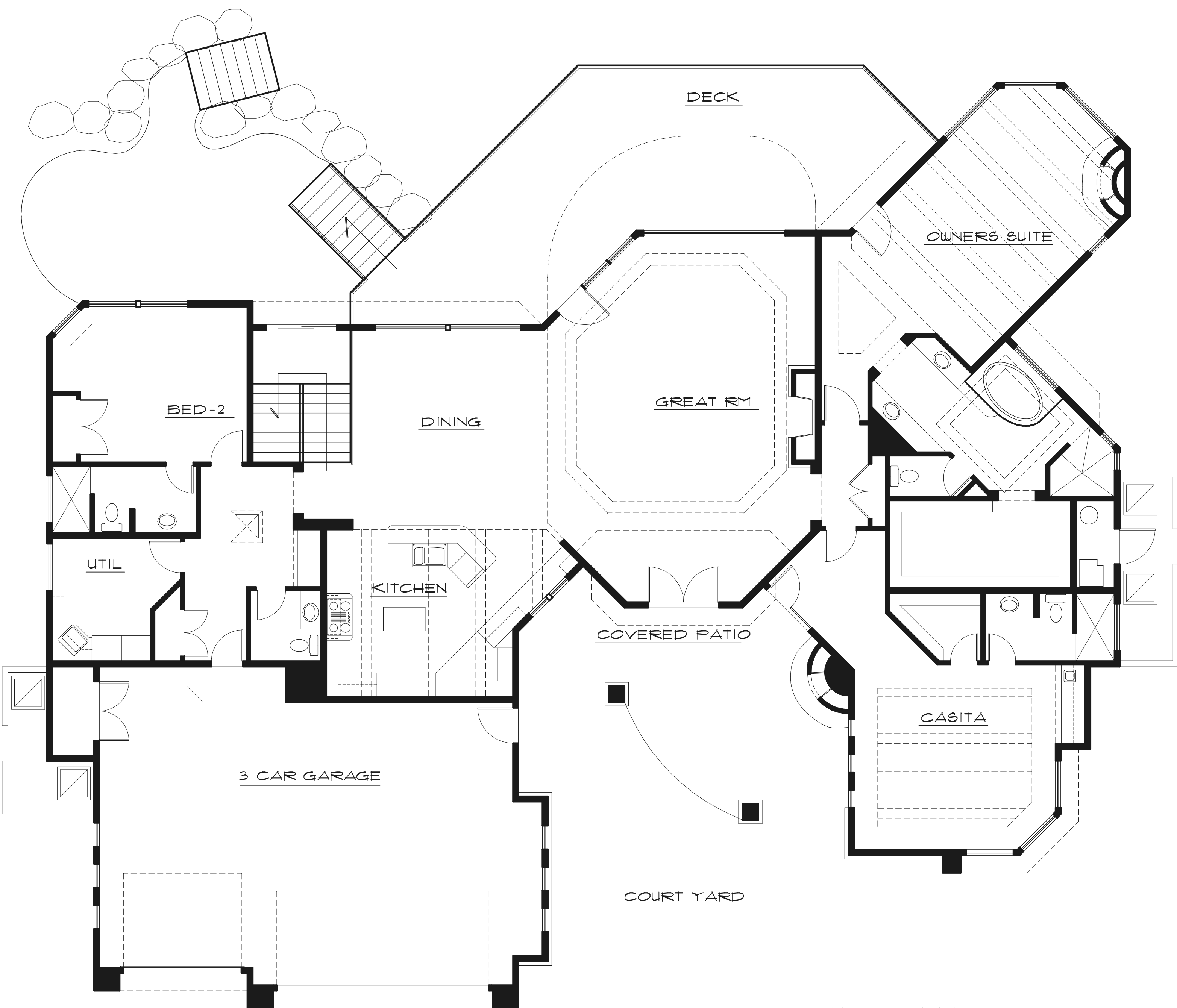
FLOOR PLAN SCALE 1/4"
